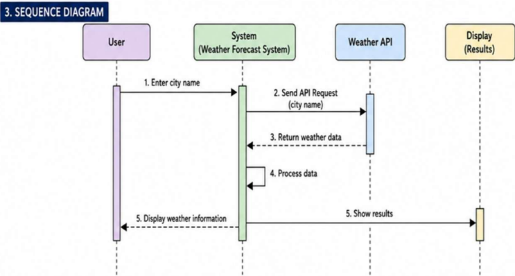
Figure: Sequence Diagram of Weather Forecast System
